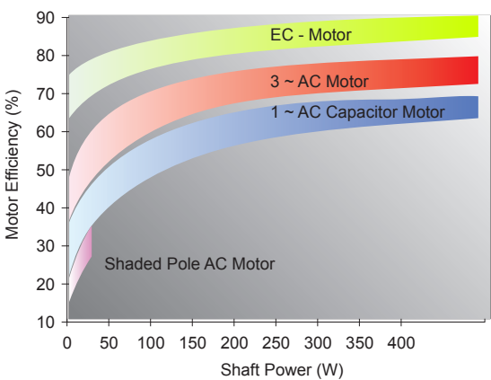
Efficiency of EC Motors Vs AC Motors
