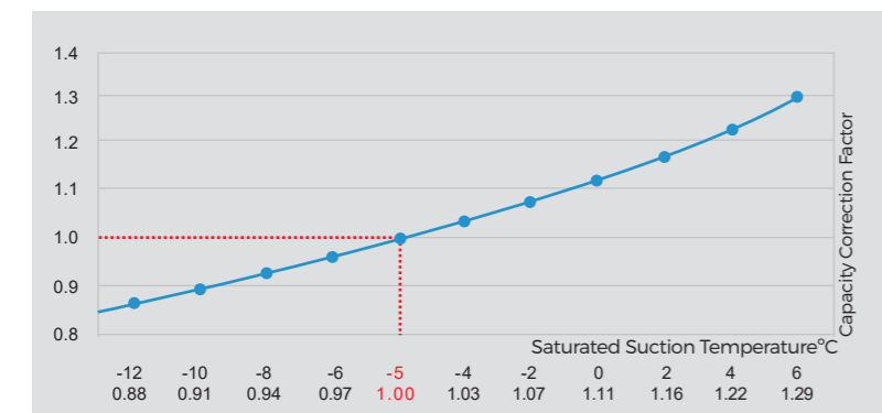
FNR Capacity Correction Graph
